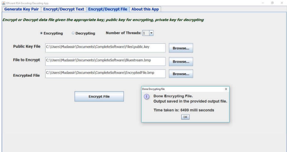
Figure 4.2 Encryption time of file size 2.25MB
