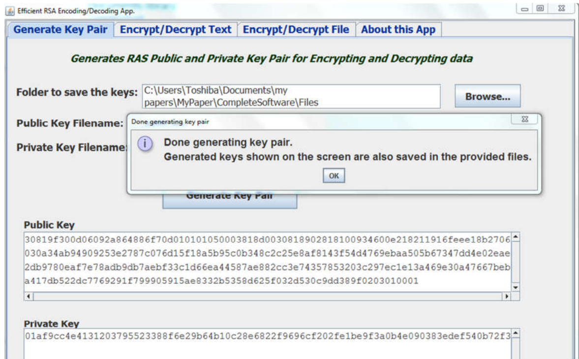
Figure 4.1 Generate key tab
